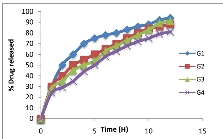
Figure 1: Cumulative in-vitro drug release of in situ gel formulations of Meloxicam
