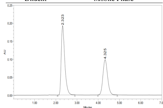
Figure 3: Typical Chromatogram of Omeprazole and Aspirin
